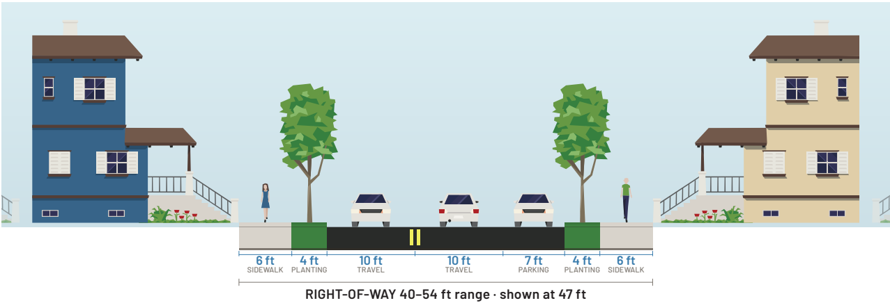
Representative section at a typical right-of-way; widths are typical values within the ranges in the Design Standards below. Cross-section illustration adapted from Streetmix (streetmix.net), © the Streetmix project, licensed CC BY-SA 4.0.
